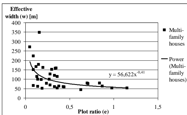
Figure 3. Effective width as a function of plot ratio in 34 district heating schemes in multi family housing districts in Sweden. Source [4]
