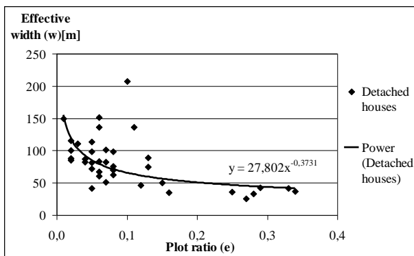
Figure 2. Effective width as a function of plot ratio in 39 district heating schemes in detached house districts in Sweden. Source: [5]
