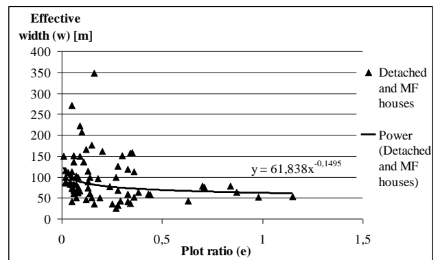
Figure 4. Effective width as a function of plot ratio, combination of 39 district heating schemes in detached house districts and 34 in multi family housing districts in Sweden. Datapoints merged from figure 2 and 3.
