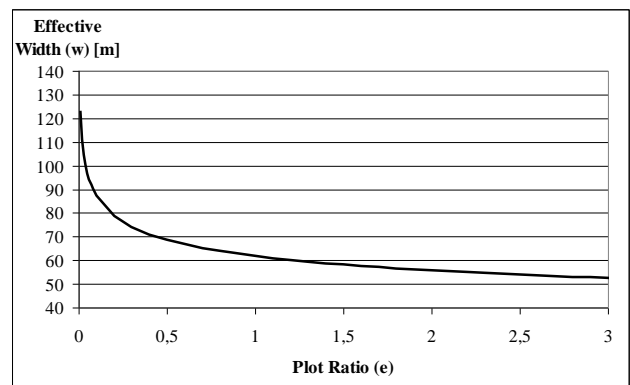
Figure 5. Effective width as a function of plot ratio by use of eq. (9).
